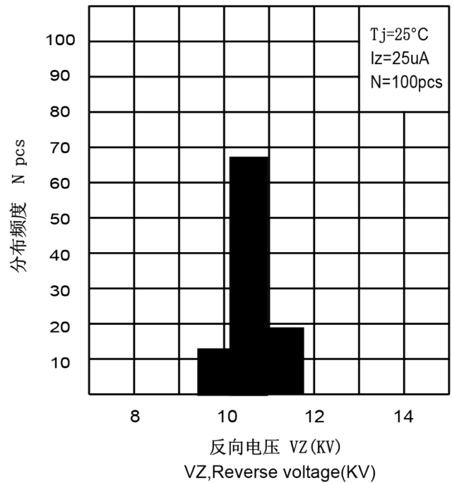
REVERSE VOLTAGE CHARACTERISTIC DISTRIBUTION
