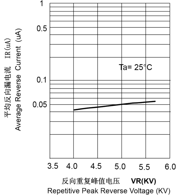
REVERSE CHARACTERISTIC [VR-IR]
