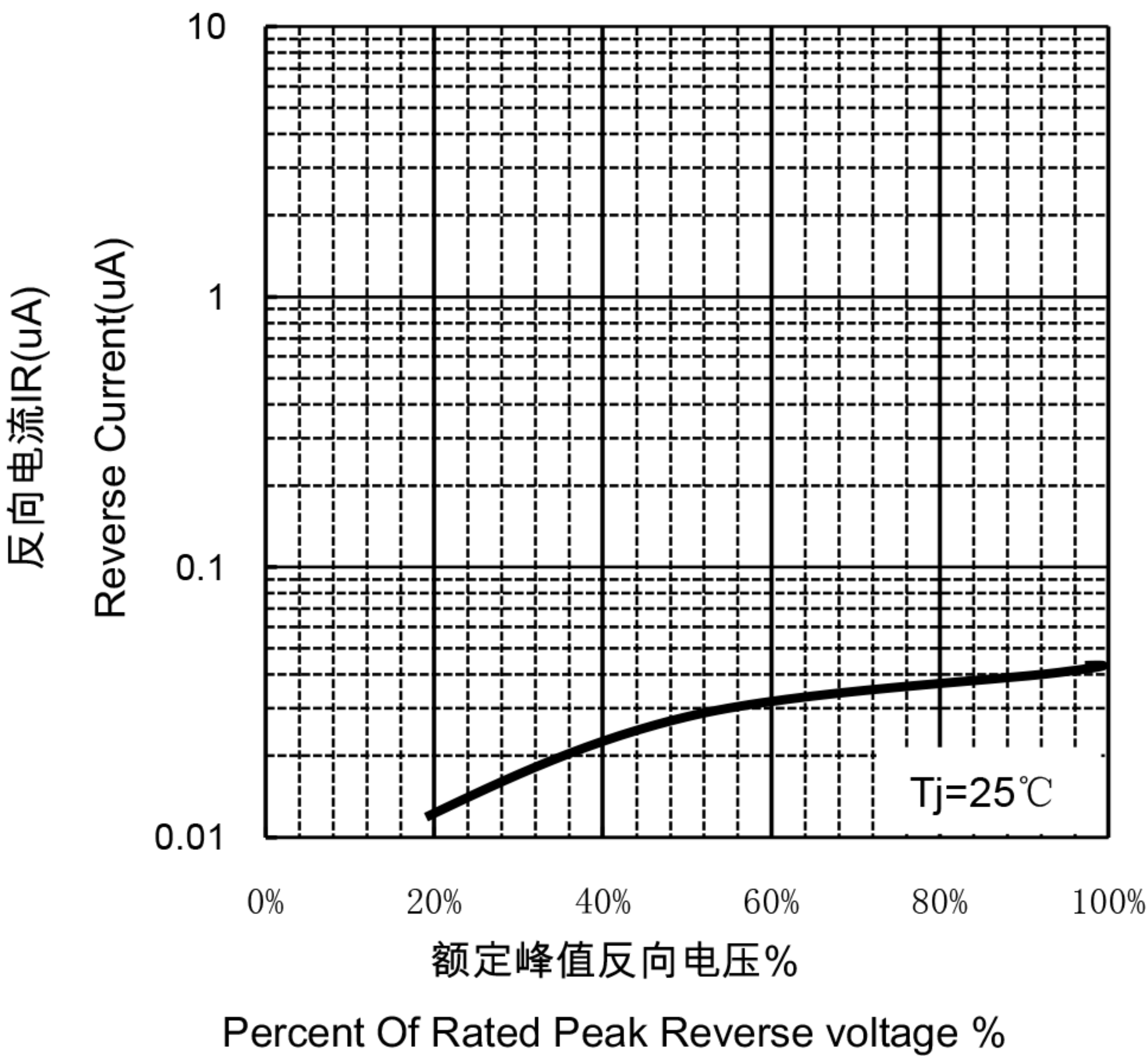
Typical Reverse Characteristics
