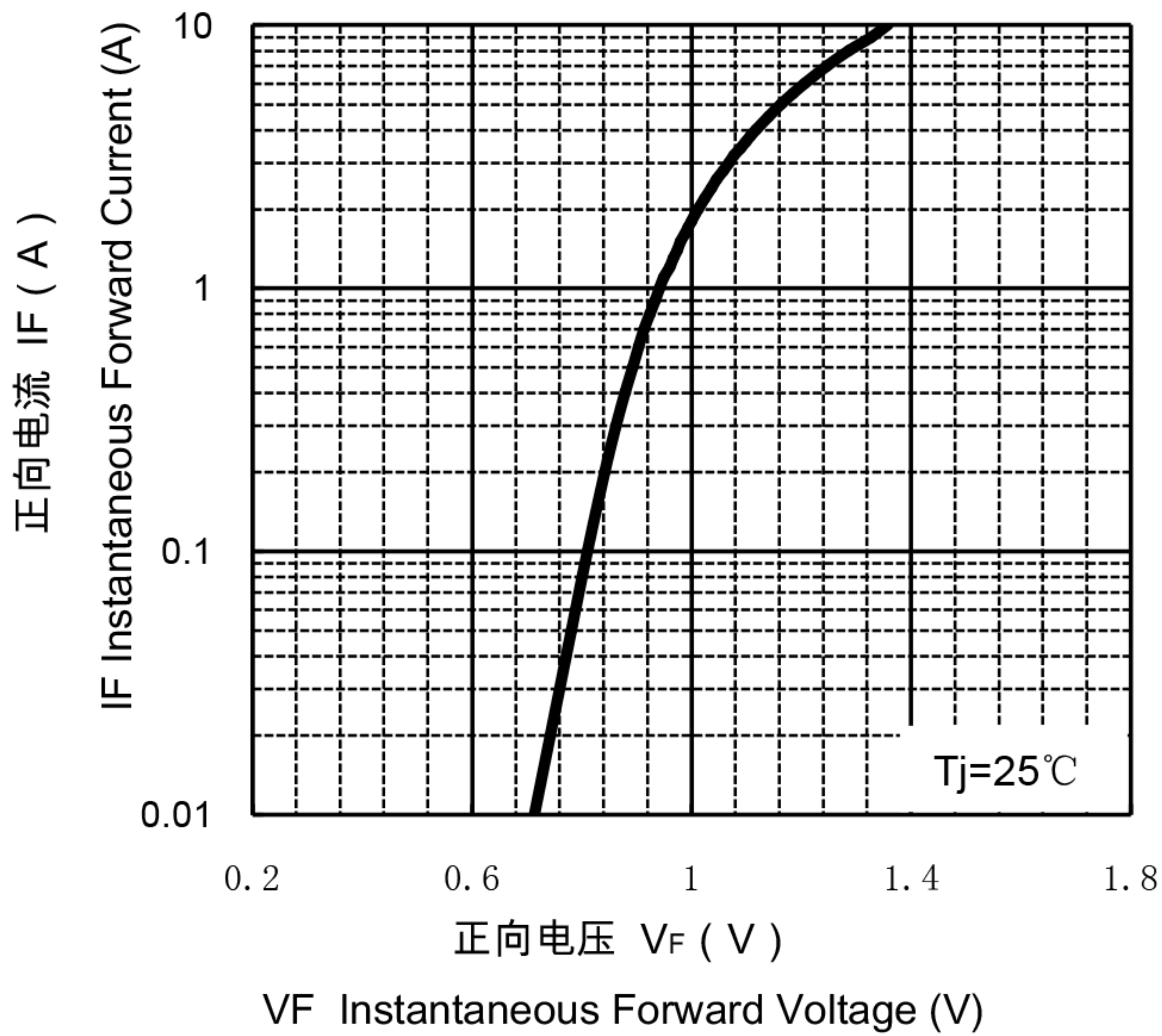
TYPICAL FORWARD CHARACTERISTIC
