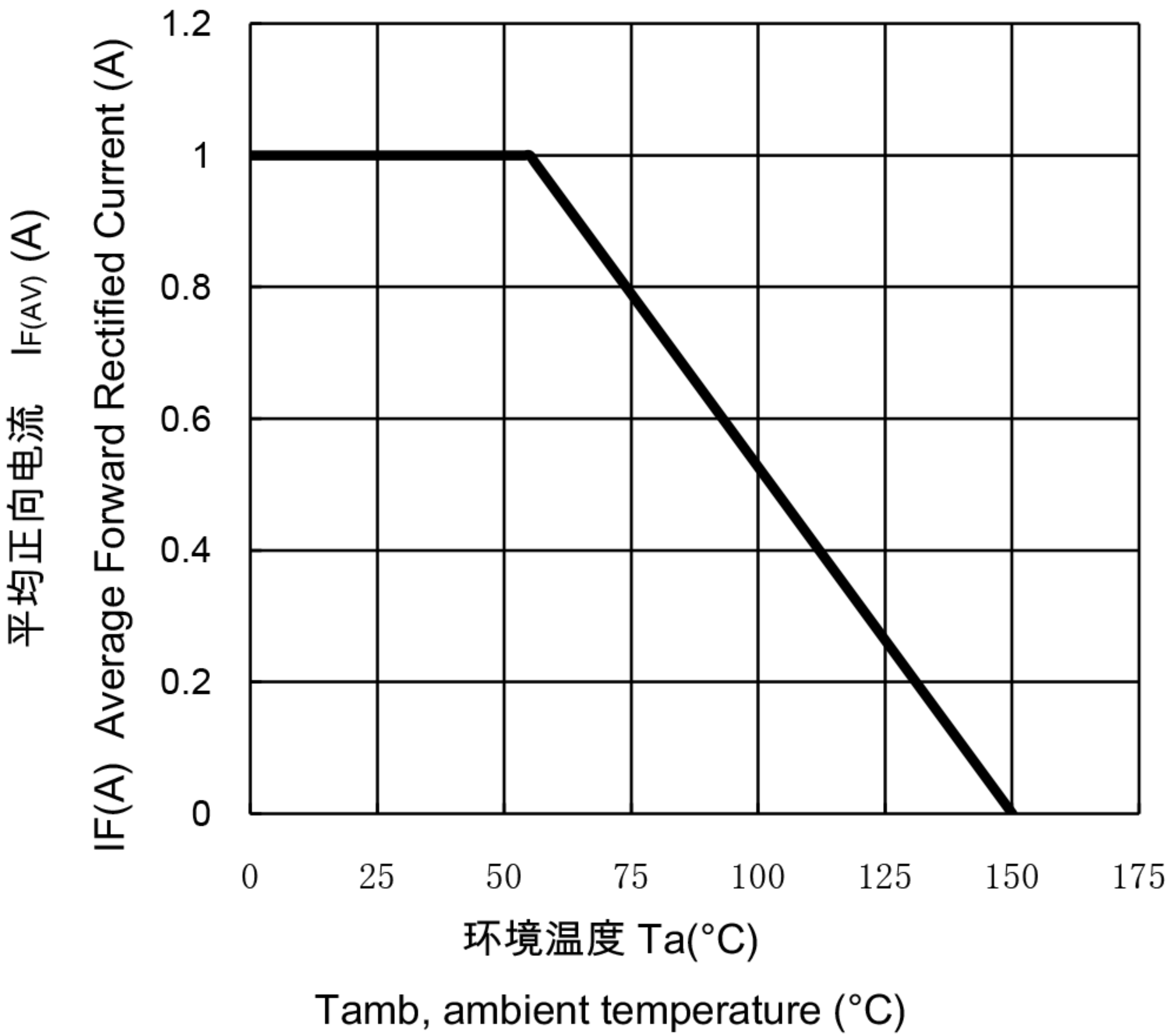
FORWARD CURRENT DERATING CURVE
