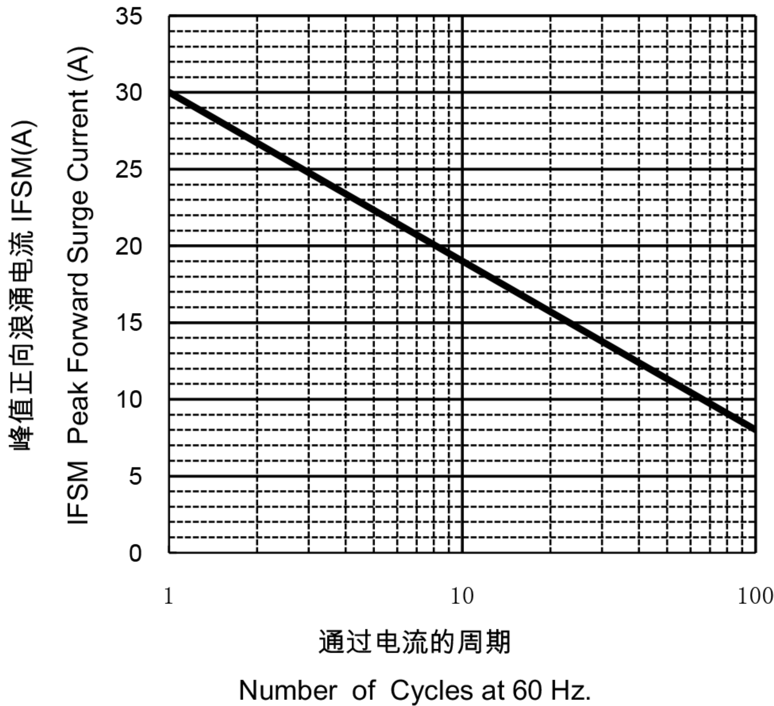
MAXIMUM NON REPETITIVE PEAK FORWARD SURGE CURRENT
